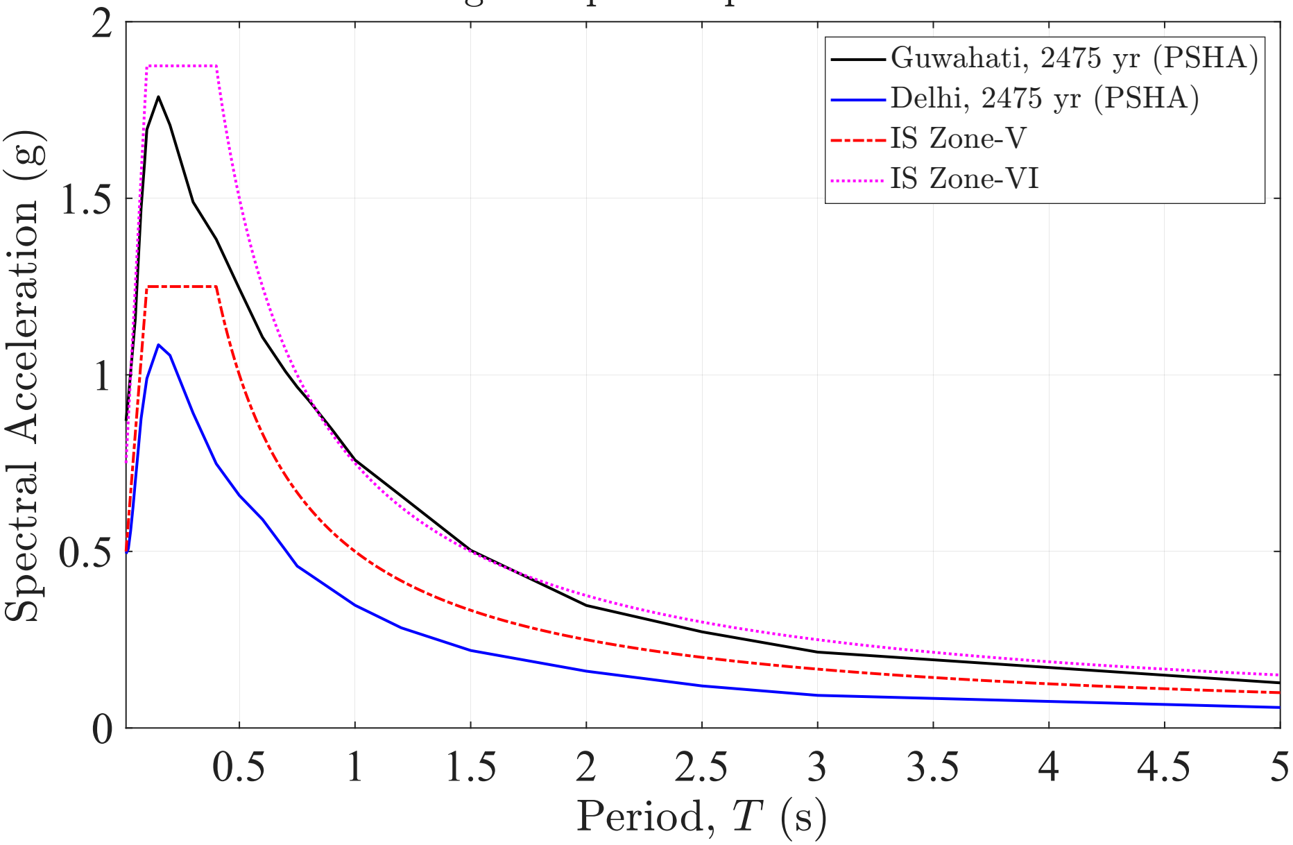
UHS and IS Design Response Spectrum - Guwahati vs Delhi
